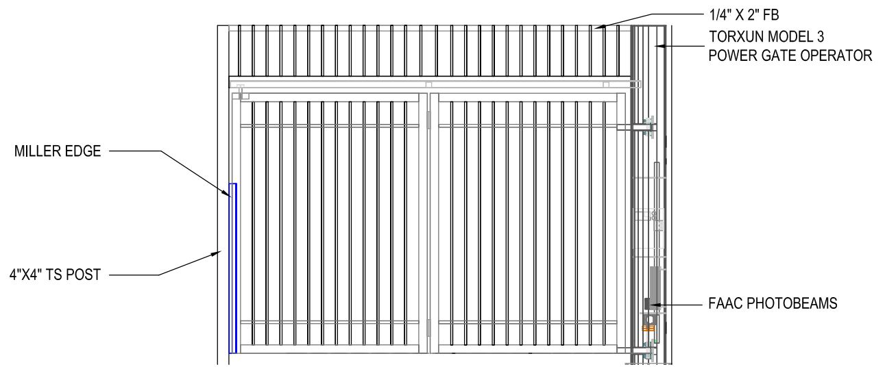
ELEVATION: BI-FOLDING SWING GATE OUTSIDE LOOKING IN
