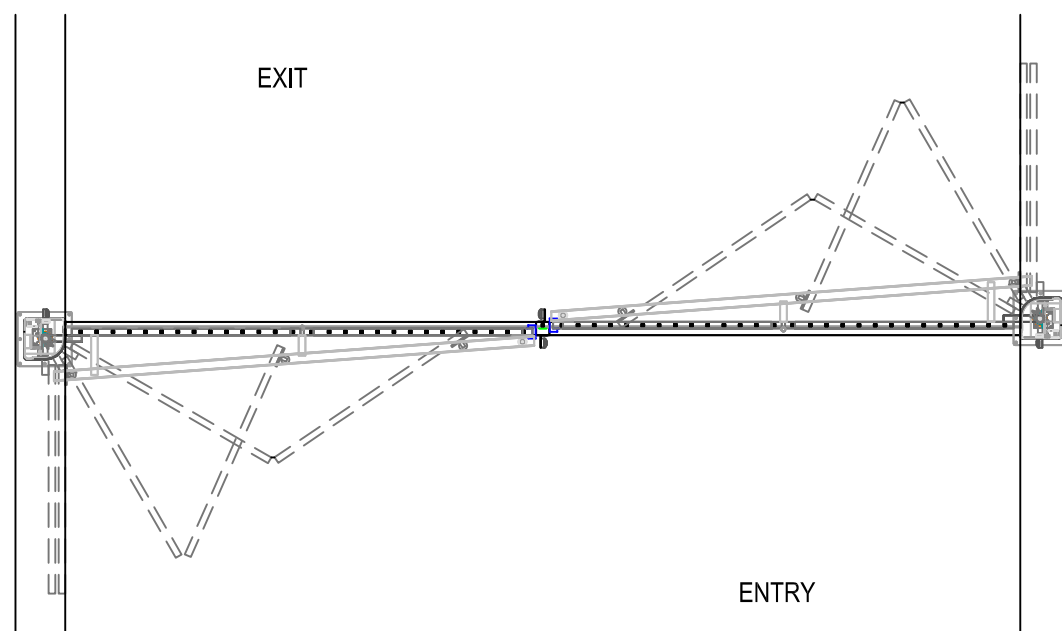
TOP VIEW: BI-FOLDING SWING GATE
