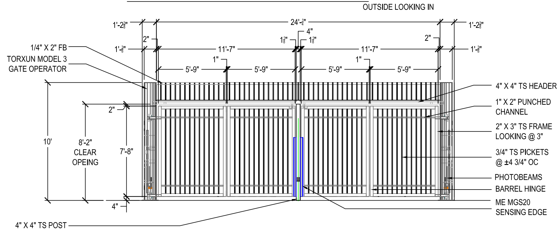
ELEVATION: BI-FOLDING SWING GATE
